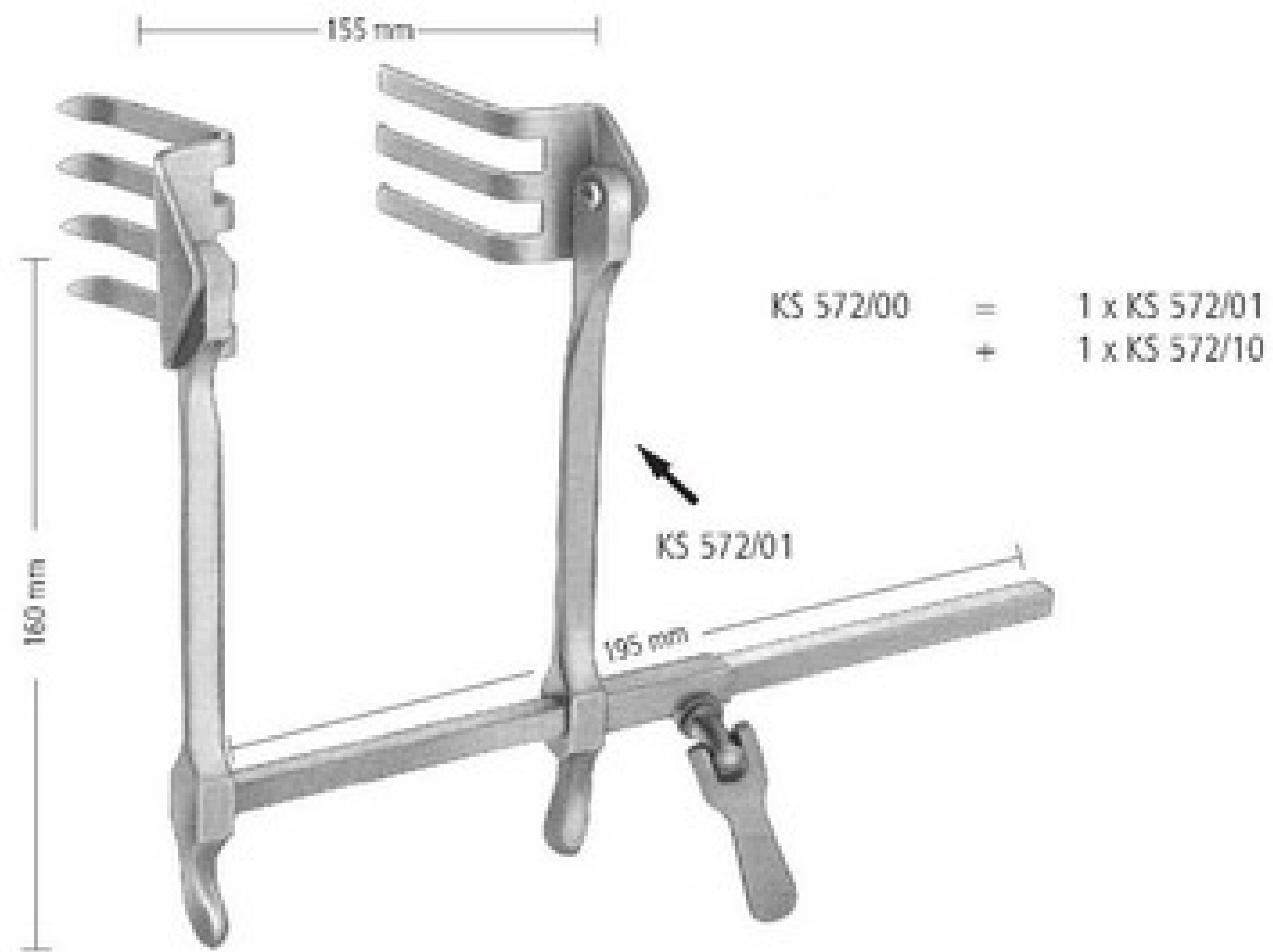
SCOVILLE-RICHTER KS 572/00
